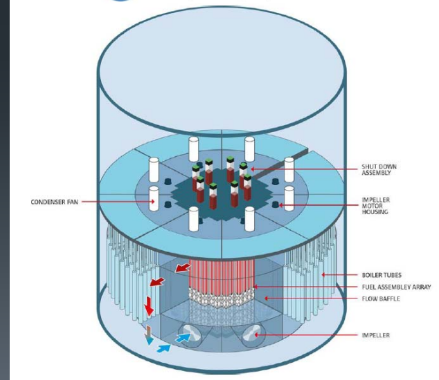
Stable Salt Reactor
